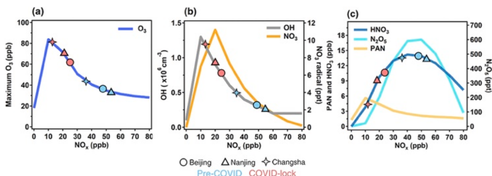
Fig. 4. (a) Box model simulated maximum O 3 concentration as a function of the initial concentrations of NO x (0–80 ppb), (b) average OH radical (grey) and NO 3 radical (yellow) concentrations, (c) average HNO 3 (dark blue), N 2 O 5 (light blue) and PAN (yellow) concentrations. Three shapes of symbols indicate the observed NO x concentrations in three sites. The blue fill symbols mean pre-COVID period and red ones represent COVID-lock period. (For interpretation of the references to colour in this figure legend, the reader is referred to the Web version of this article.)
